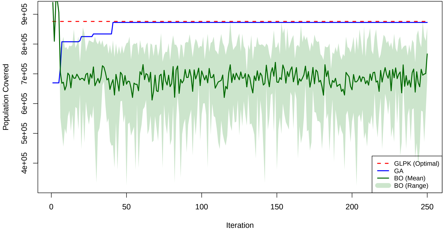
Convergence Comparison: GLPK vs GA vs BO (Trial 1)
